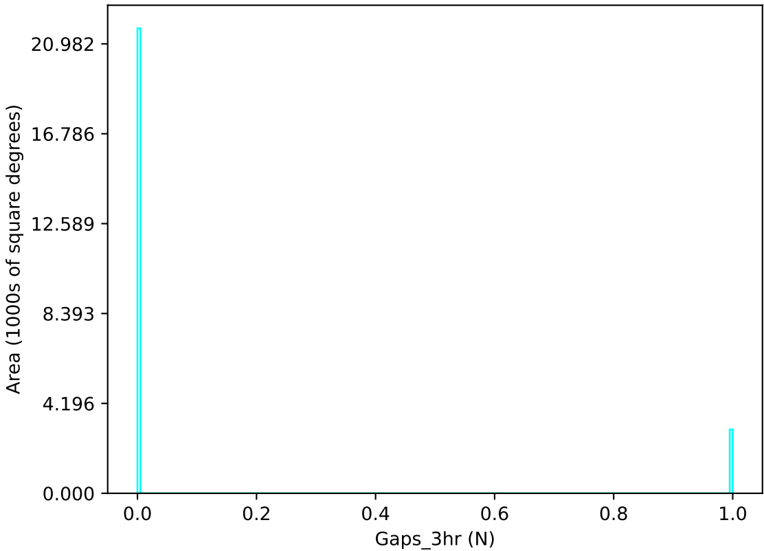
ddf_acor_sf15_lsf30_lsr10_v3.4_10yrs u band: Gaps_3hr
