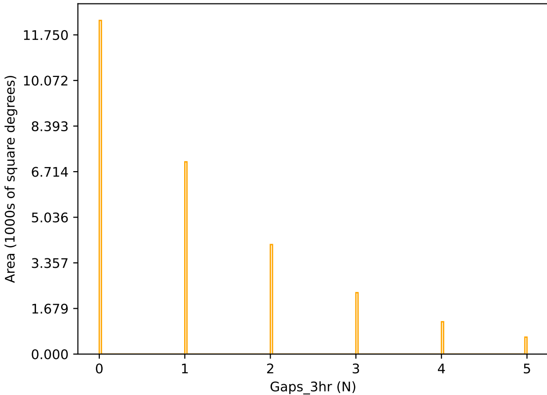
ddf_acor_sf15_lsf30_lsr10_v3.4_10yrs r band: Gaps_3hr
