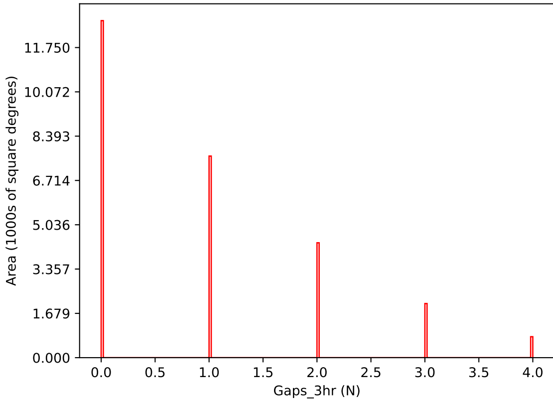
ddf_acor_sf15_lsf30_lsr10_v3.4_10yrs i band: Gaps_3hr
