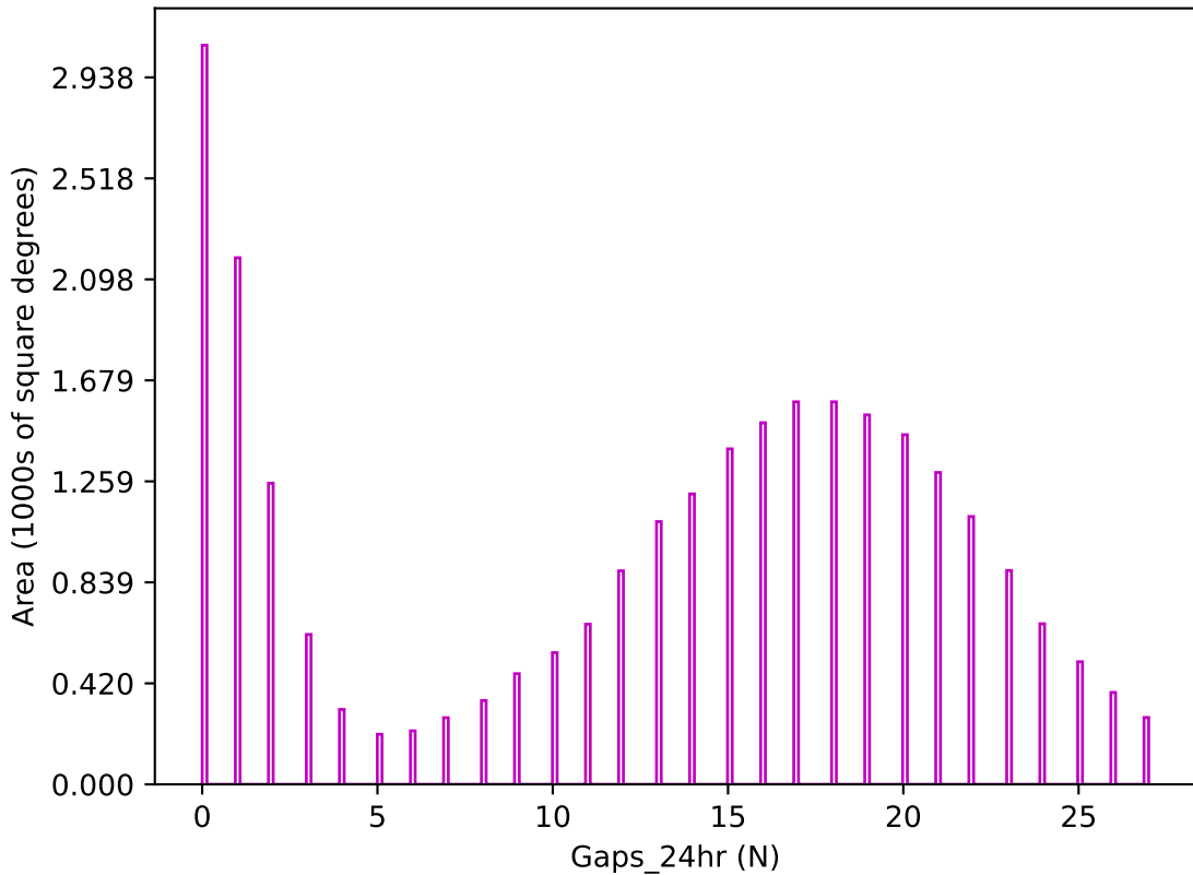
ddf_acor_sf15_ls30_lsr10_v3.4_10yrs z band: Gaps_24hr
