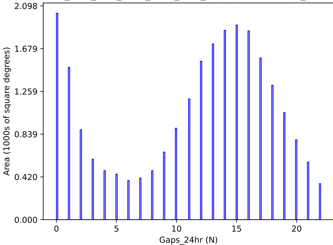
ddf_acor_sf15_lsf30_lsr10_v3.4_10yrs y band: Gaps_24hr
