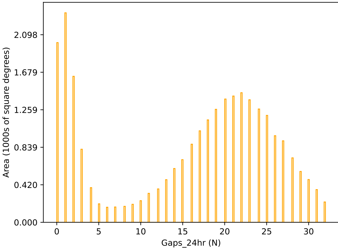
ddf_acor_sf15_ls30_lsr10_v3.4_10yrs r band: Gaps_24hr
