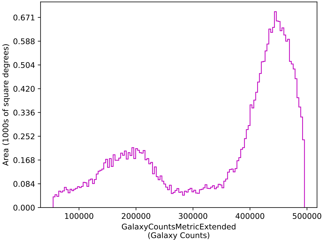
ddf_acor_sf15_lsf30_lsr10_v3.4_10yrs z: GalaxyCountsMetricExtended
