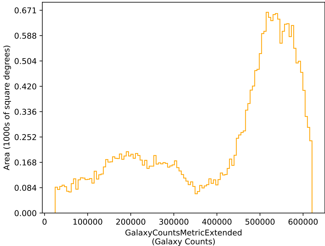
ddf_acor_sf15_lsf30_lsr10_v3.4_10yrs r: GalaxyCountsMetricExtended
