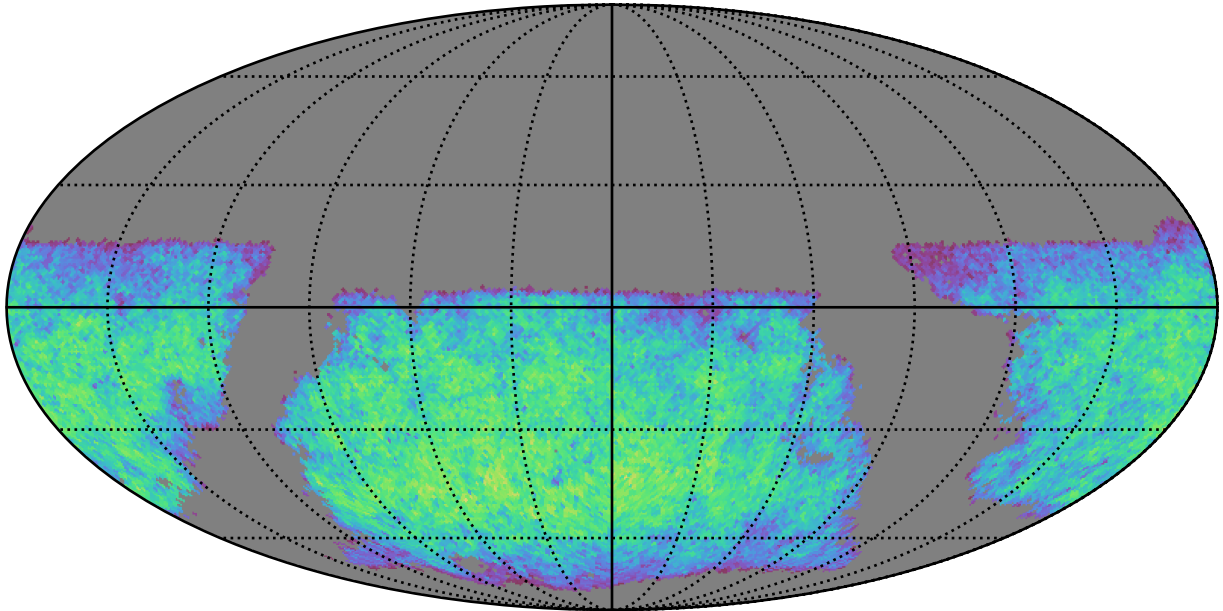
ddf_acor_sf15_lsf30_lsr10_v3.4_10yrs i band non-DD year 1: ExgalM5WithCuts
