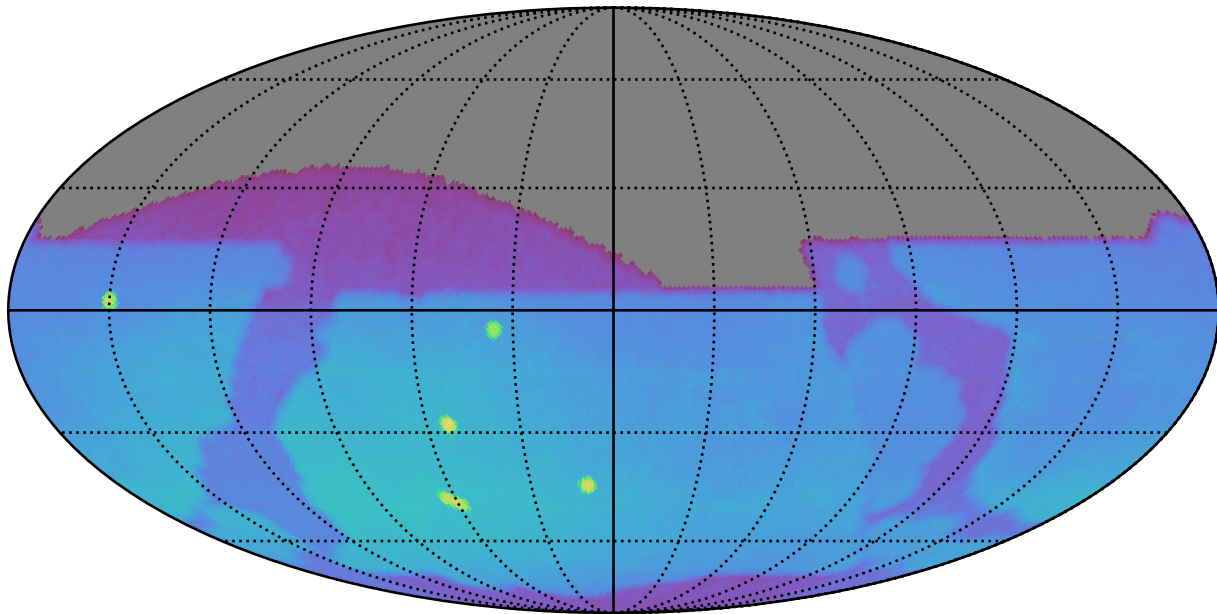
ddf_acor_sf15_lsf30_lsr10_v3.4_10yrs : Brown Dwarf, L7
