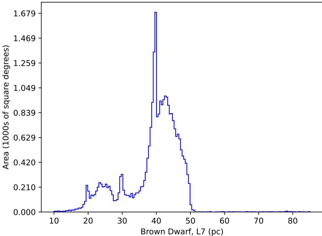
ddf_acor_sf15_lsf30_lsr10_v3.4_10yrs : Brown Dwarf, L7
