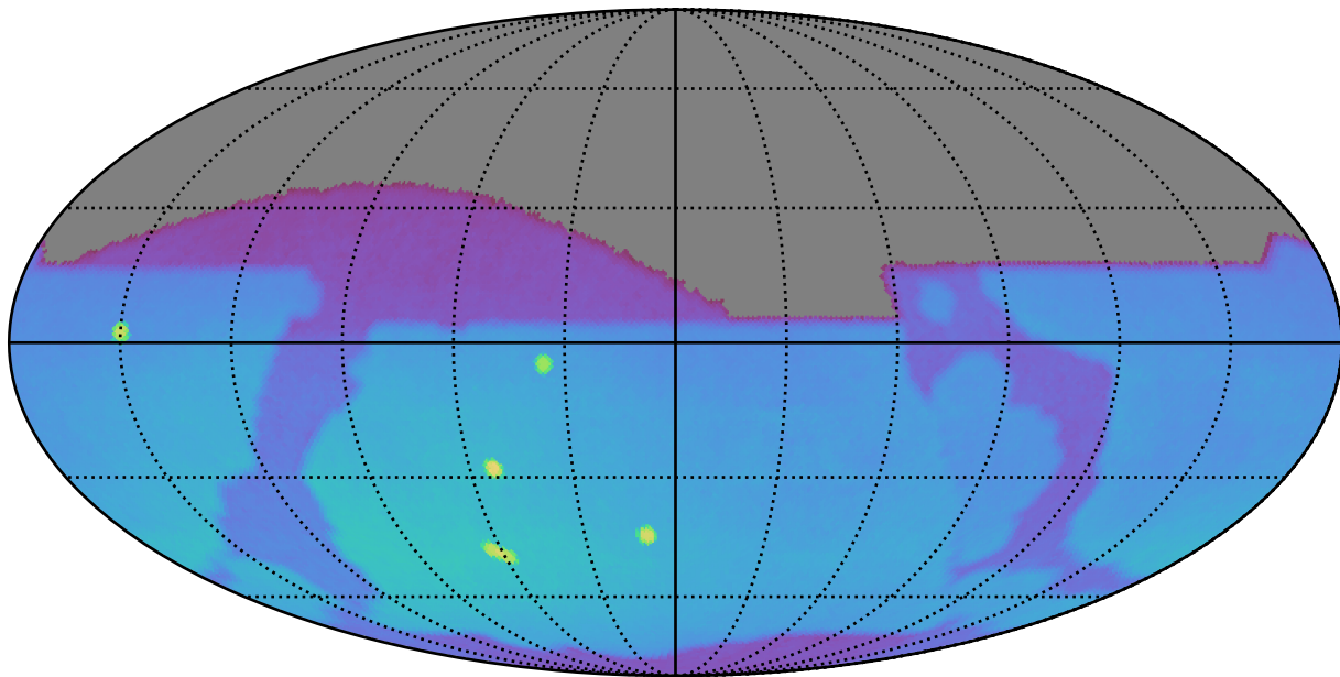
ddf_acor_sf15_lsf30_lsr10_v3.4_10yrs : Brown Dwarf, L4
