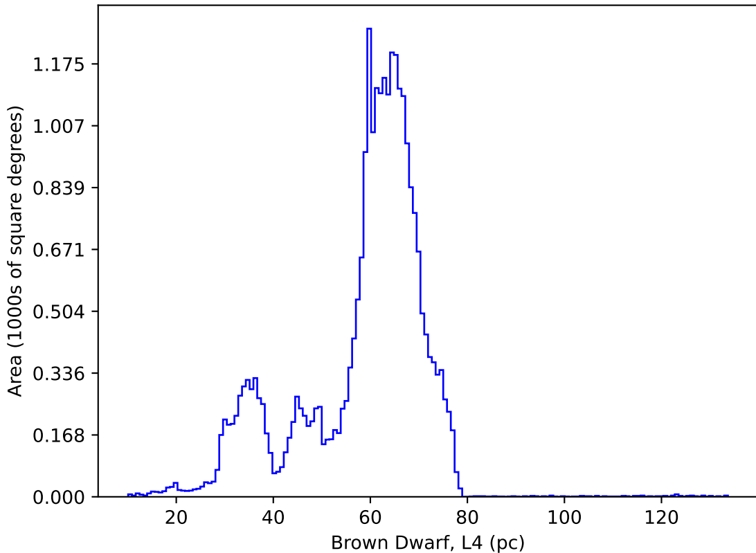
ddf_acor_sf15_lsf30_lsr10_v3.4_10yrs : Brown Dwarf, L4
