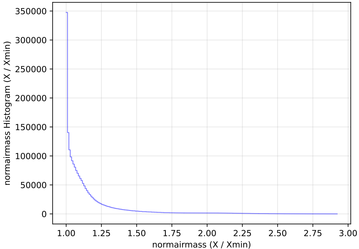
ddf_acor_sf15_lsf30_lsr10_v3.4_10yrs WFD all bands: normairmass Histogram
