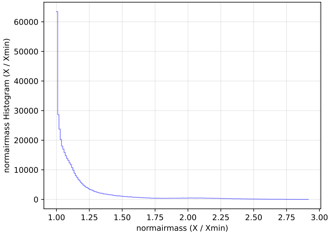
ddf_acor_sf15_lsf30_lsr10_v3.4_10yrs All sky z band: normairmass Histogram
