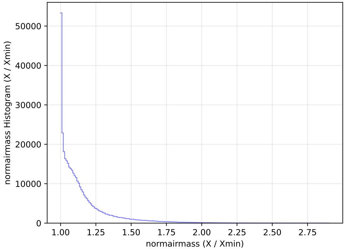
ddf_acor_sf15_lsf30_lsr10_v3.4_10yrs All sky y band: normairmass Histogram
