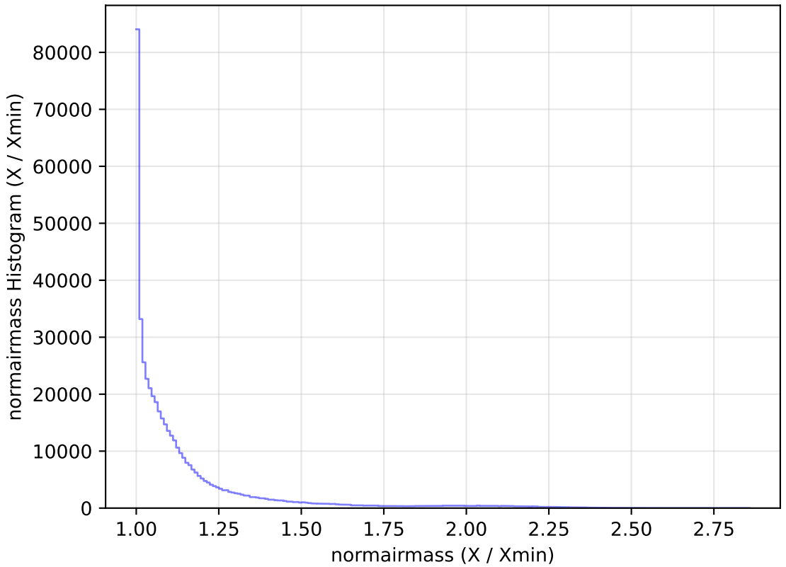
ddf_acor_sf15_lsf30_lsr10_v3.4_10yrs All sky r band: normairmass Histogram
