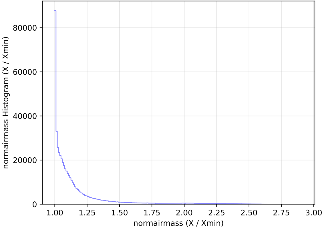
ddf_acor_sf15_lsf30_lsr10_v3.4_10yrs All sky i band: normairmass Histogram
