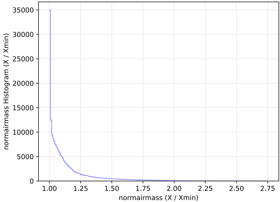
ddf_acor_sf15_lsf30_lsr10_v3.4_10yrs All sky g band: normairmass Histogram
