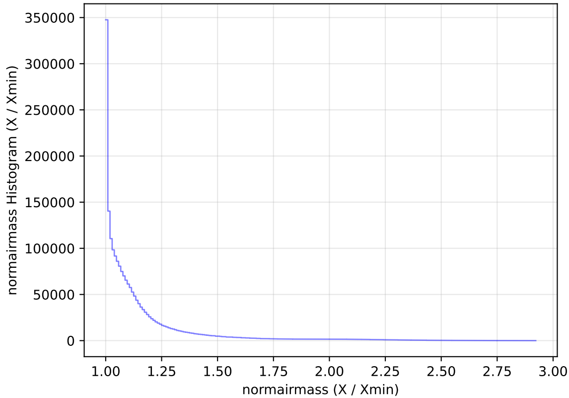
ddf_acor_sf15_lsf30_lsr10_v3.4_10yrs All sky all bands: normairmass Histogram
