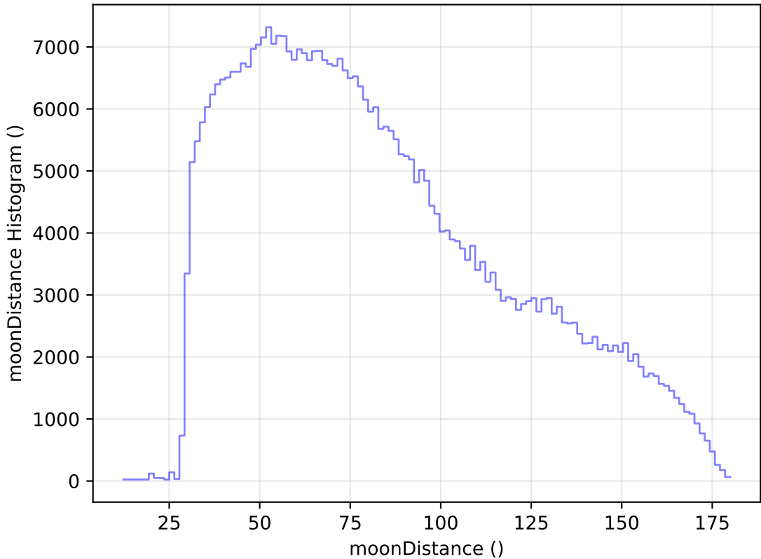
ddf_acor_sf15_lsf30_lsr10_v3.4_10yrs WFD z band: moonDistance Histogram
