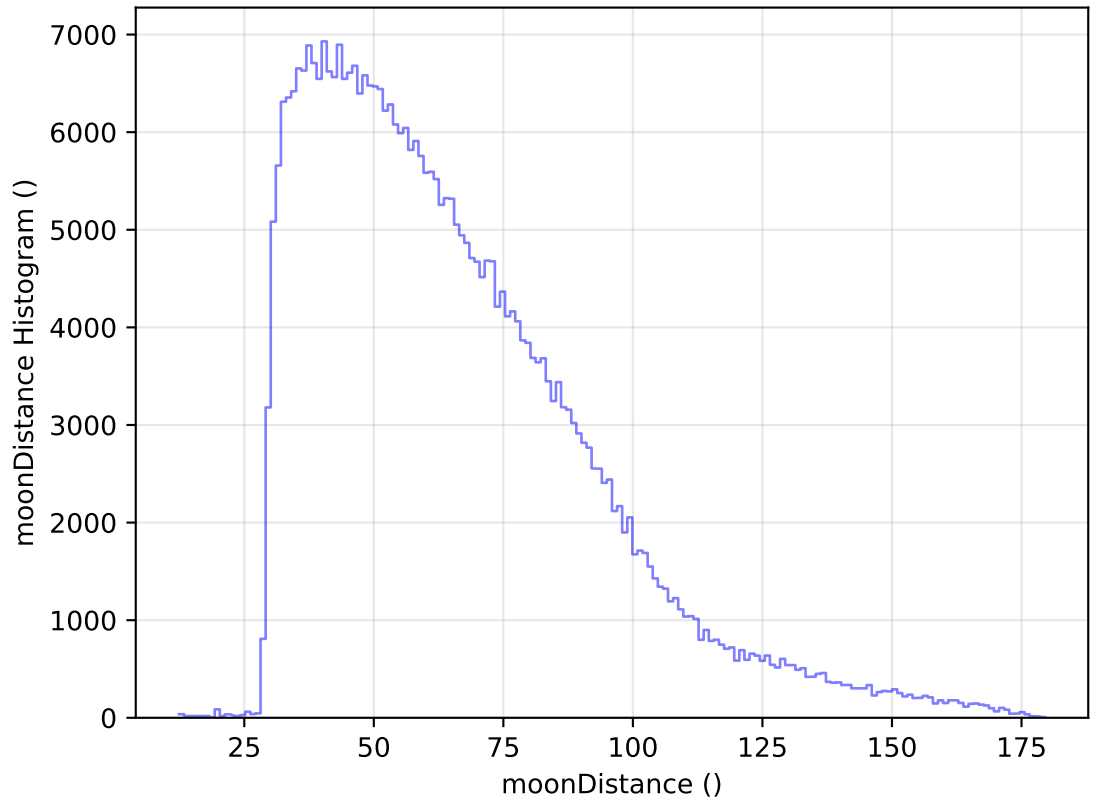
ddf_acor_sf15_Isf30_Isr10_v3.4_10yrs WFD y band: moonDistance Histogram
