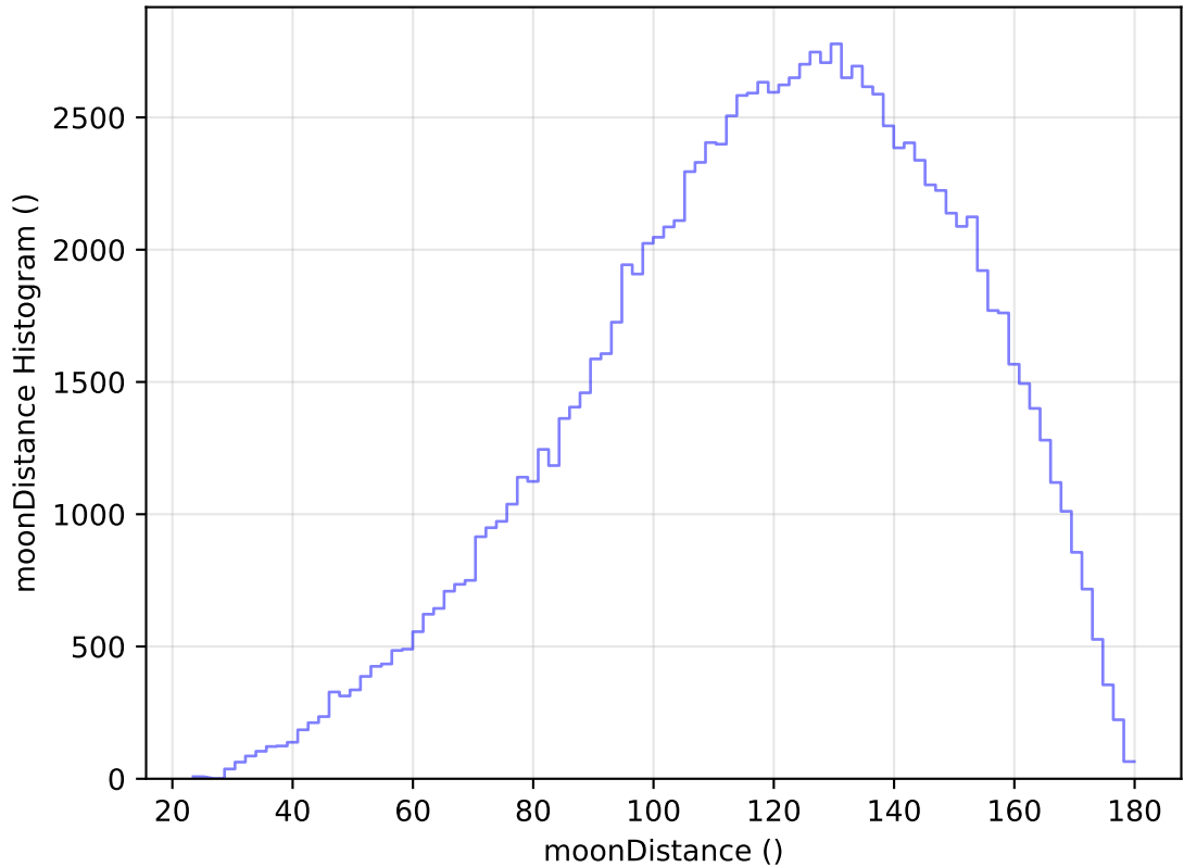
ddf_acor_sf15_lsf30_lsr10_v3.4_10yrs WFD u band: moonDistance Histogram
