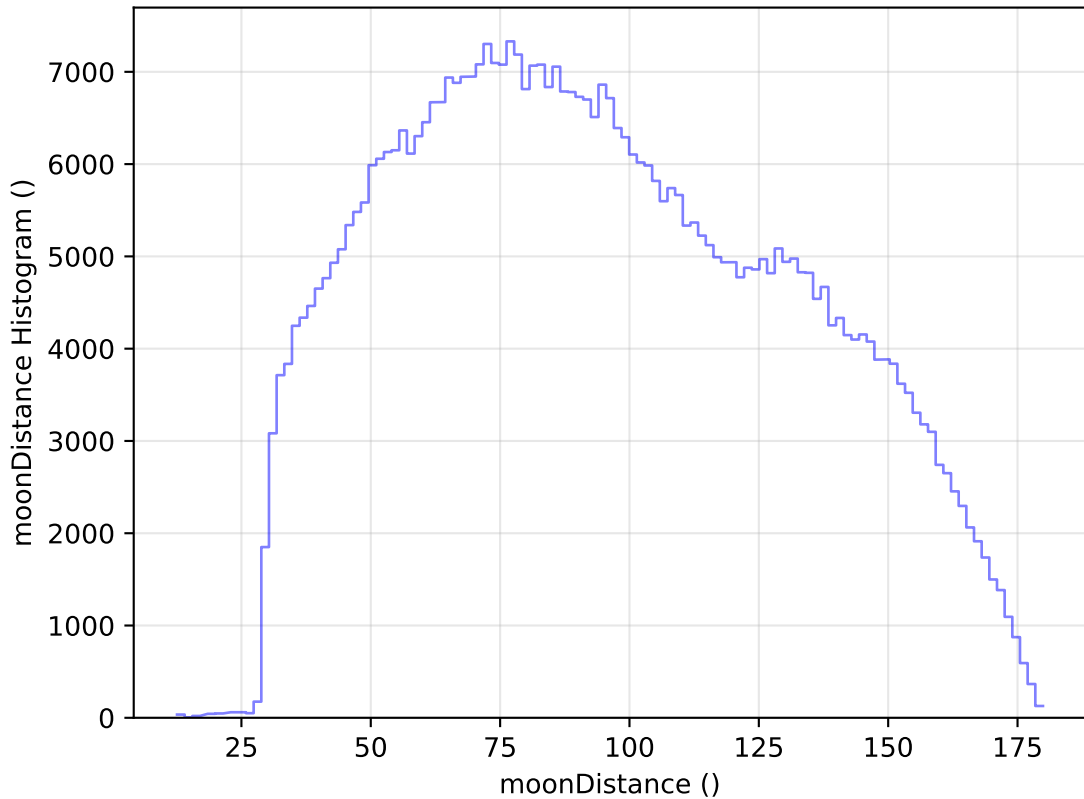
ddf_acor_sf15_lsf30_lsr10_v3.4_10yrs WFD i band: moonDistance Histogram
