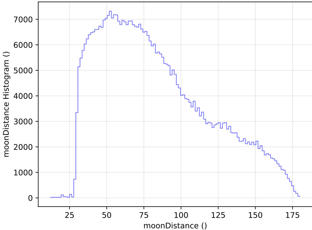
ddf_acor_sf15_lsf30_lsr10_v3.4_10yrs All sky z band: moonDistance Histogram
