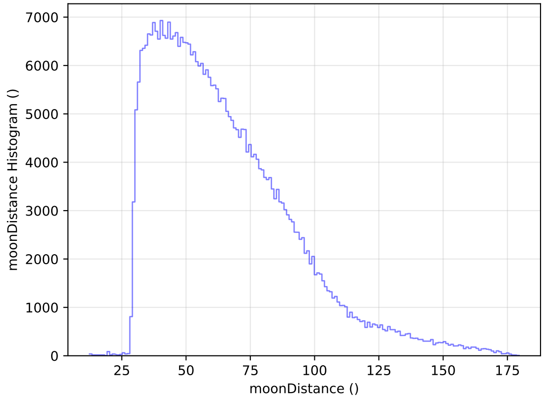
ddf_acor_sf15_lsf30_lsr10_v3.4_10yrs All sky y band: moonDistance Histogram
