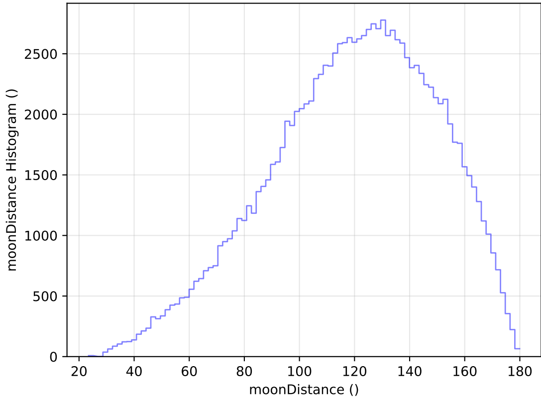
ddf_acor_sf15_lsf30_lsr10_v3.4_10yrs All sky u band: moonDistance Histogram
