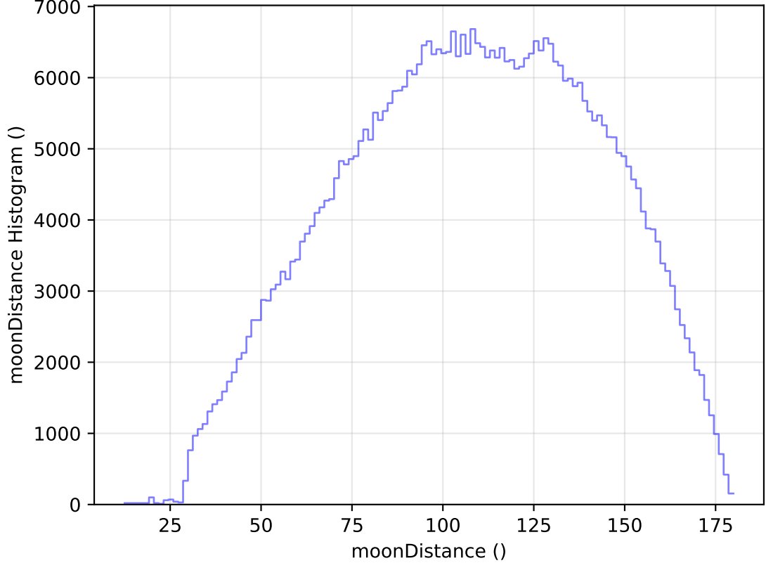
ddf_acor_sf15_lsf30_lsr10_v3.4_10yrs All sky r band: moonDistance Histogram
