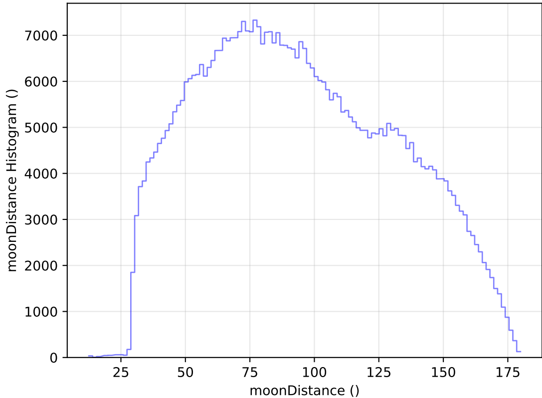
ddf_acor_sf15_lsf30_lsr10_v3.4_10yrs All sky i band: moonDistance Histogram
