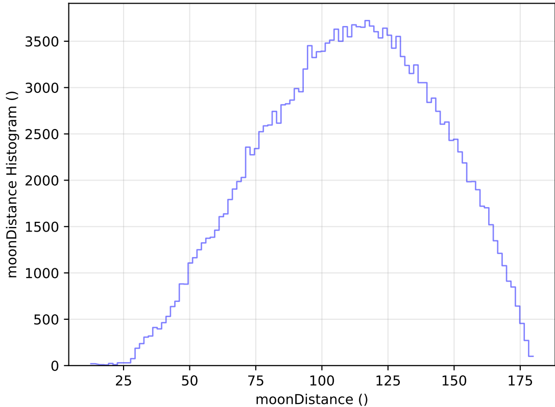
ddf_acor_sf15_lsf30_lsr10_v3.4_10yrs All sky g band: moonDistance Histogram
