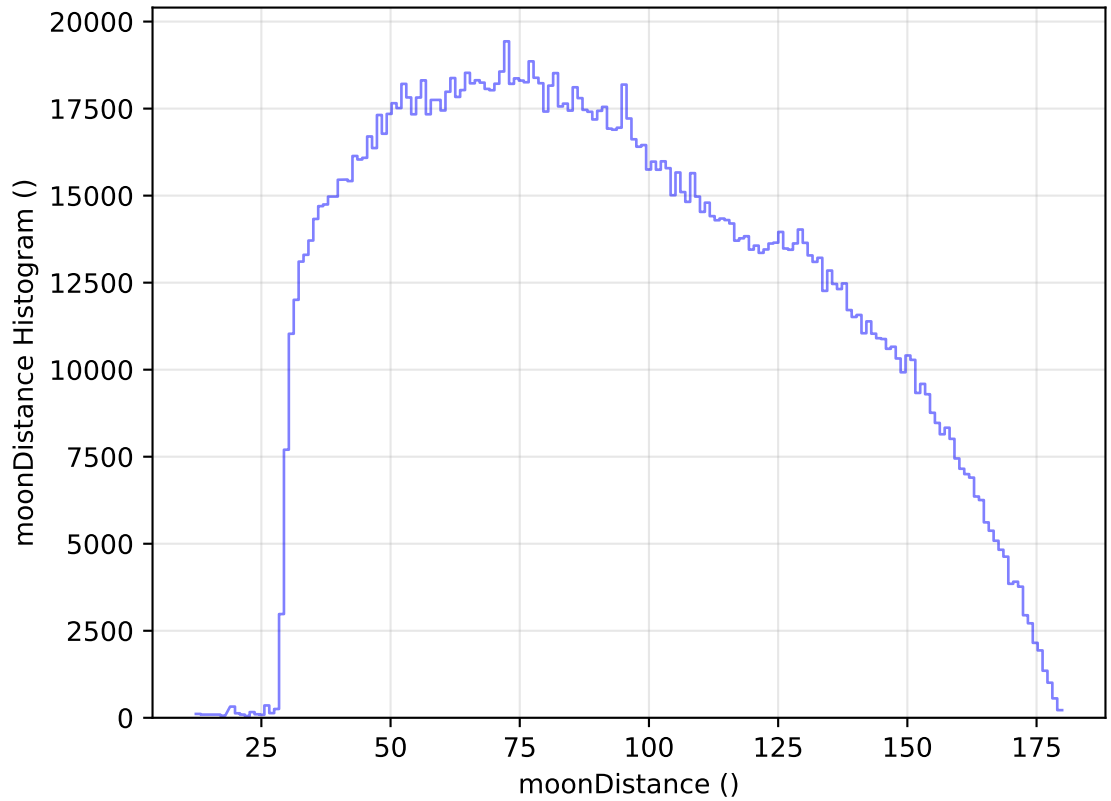
ddf_acor_sf15_lsf30_lsr10_v3.4_10yrs All sky all bands: moonDistance Histogram
