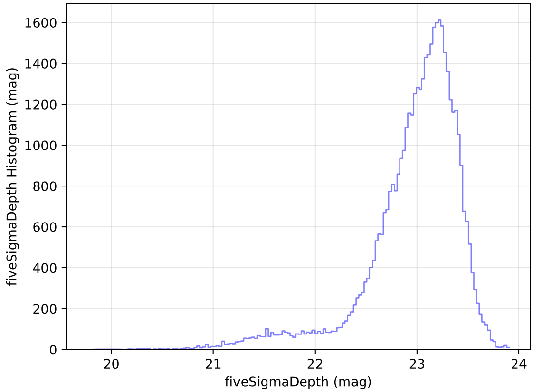
ddf_acor_sf15_lsf30_lsr10_v3.4_10yrs Yr 1 z band: fiveSigmaDepth Histogram
