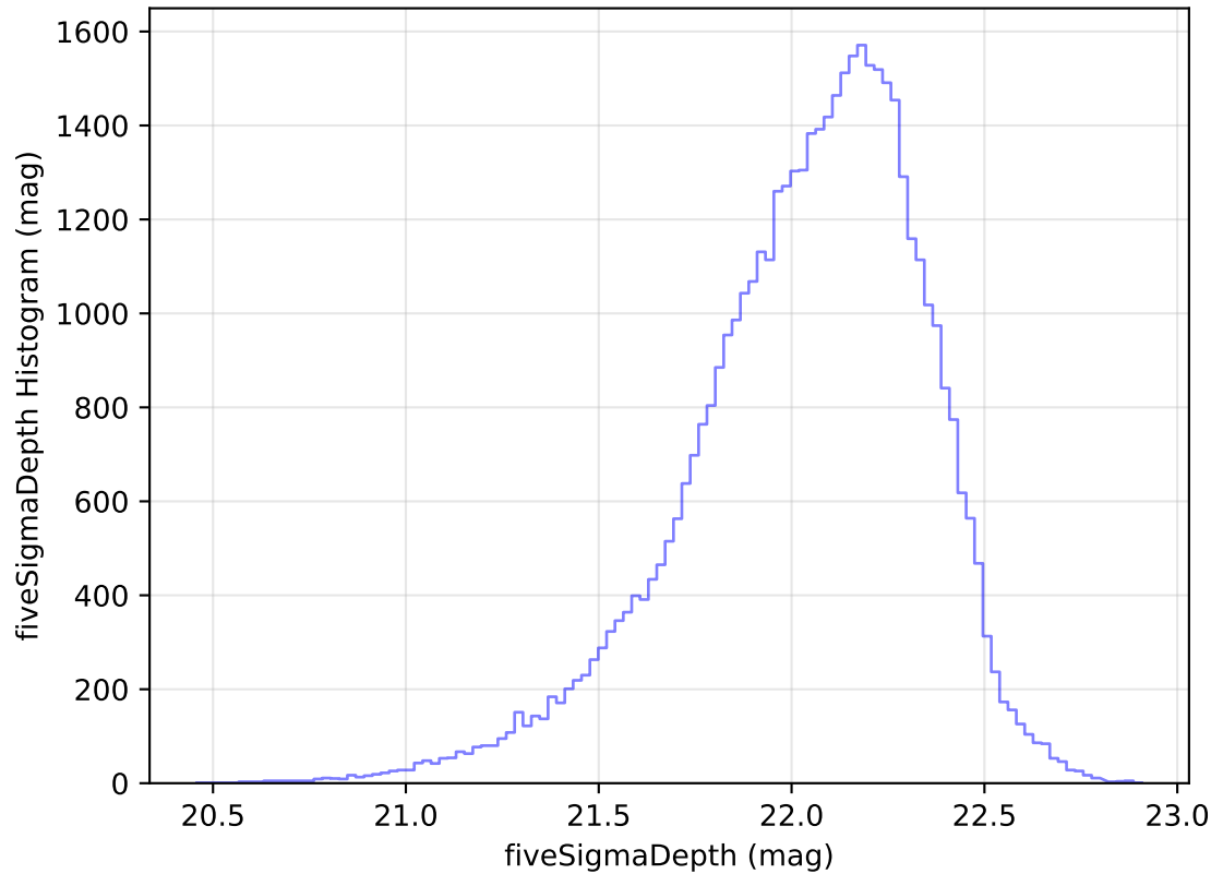
ddf_acor_sf15_lsf30_lsr10_v3.4_10yrs Yr 1 y band: fiveSigmaDepth Histogram
