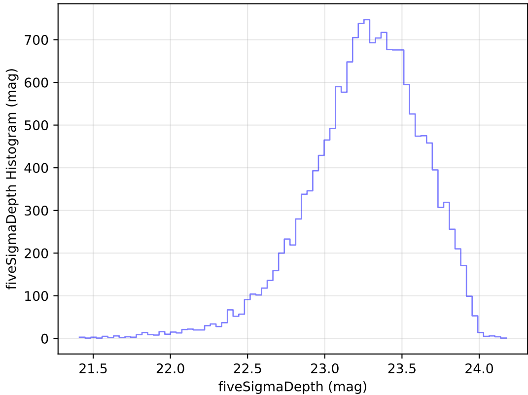
ddf_acor_sf15_lsf30_lsr10_v3.4_10yrs Yr 1 u band: fiveSigmaDepth Histogram
