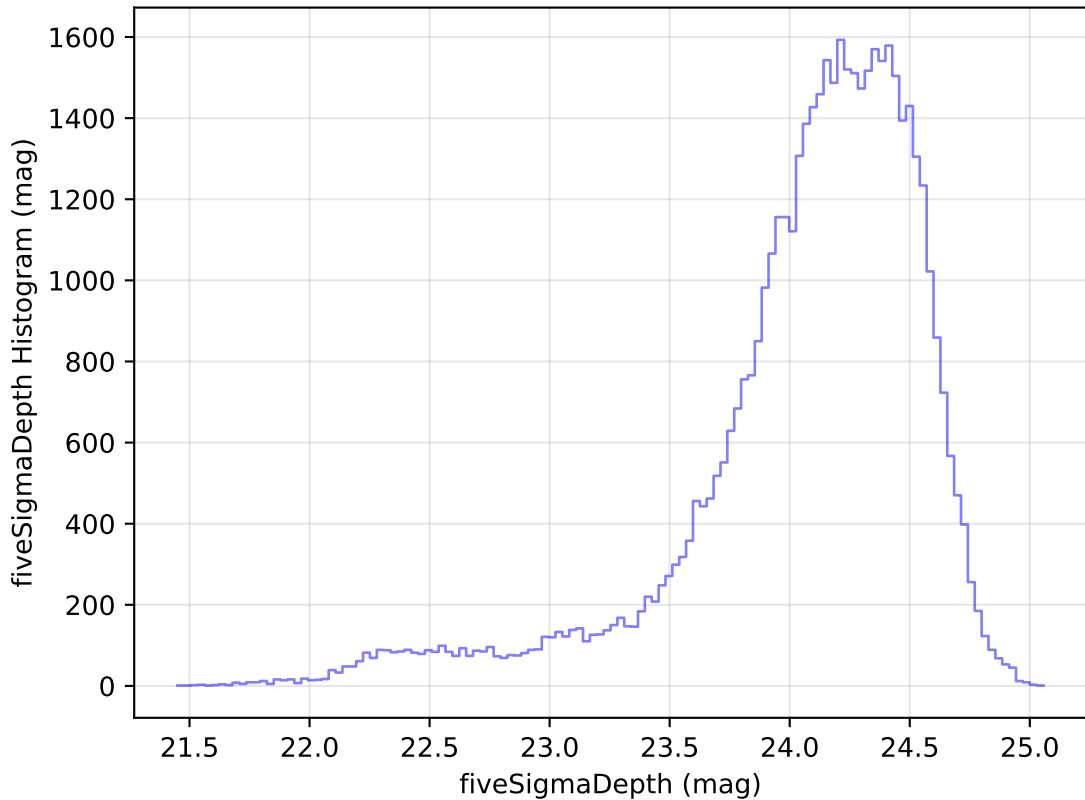
ddf_acor_sf15_lsf30_lsr10_v3.4_10yrs Yr 1 r band: fiveSigmaDepth Histogram
