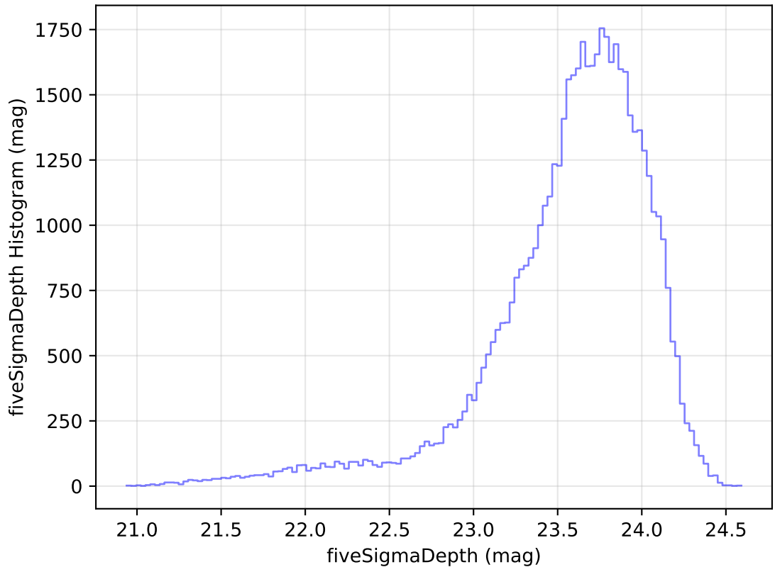
ddf_acor_sf15_lsf30_lsr10_v3.4_10yrs Yr 1 i band: fiveSigmaDepth Histogram
