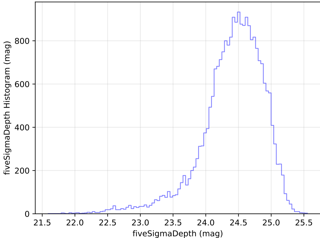
ddf_acor_sf15_lsf30_lsr10_v3.4_10yrs Yr 1 g band: fiveSigmaDepth Histogram
