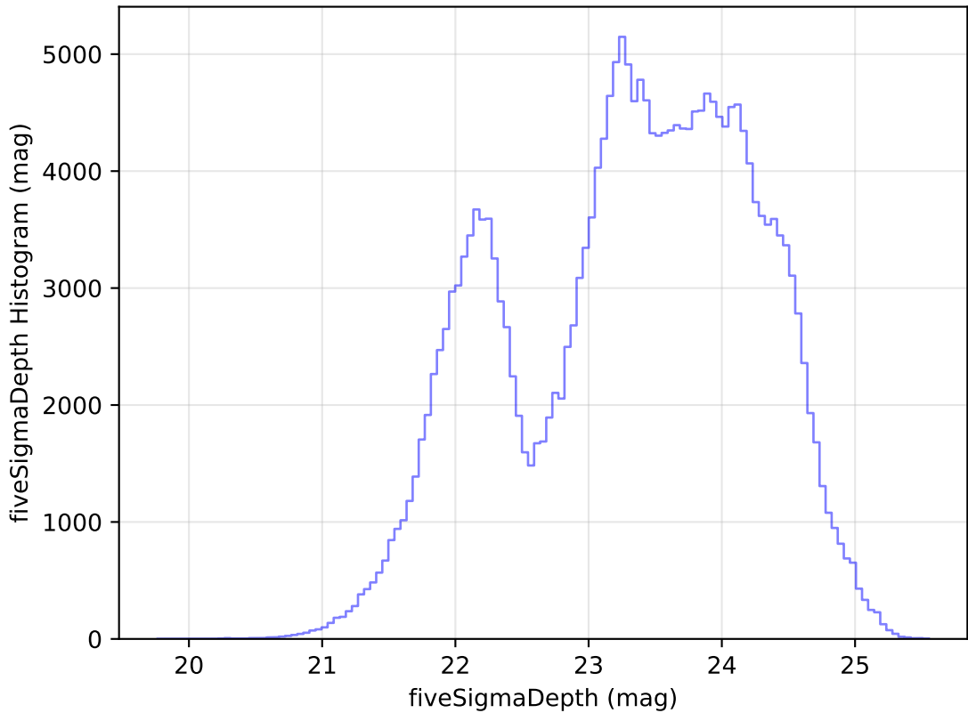
ddf_acor_sf15_Isf30_Isr10_v3.4_10yrs Yr 1 all bands: fiveSigmaDepth Histogram
