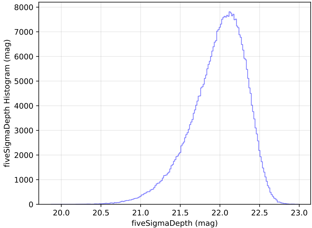
ddf_acor_sf15_lsf30_lsr10_v3.4_10yrs WFD y band: fiveSigmaDepth Histogram
