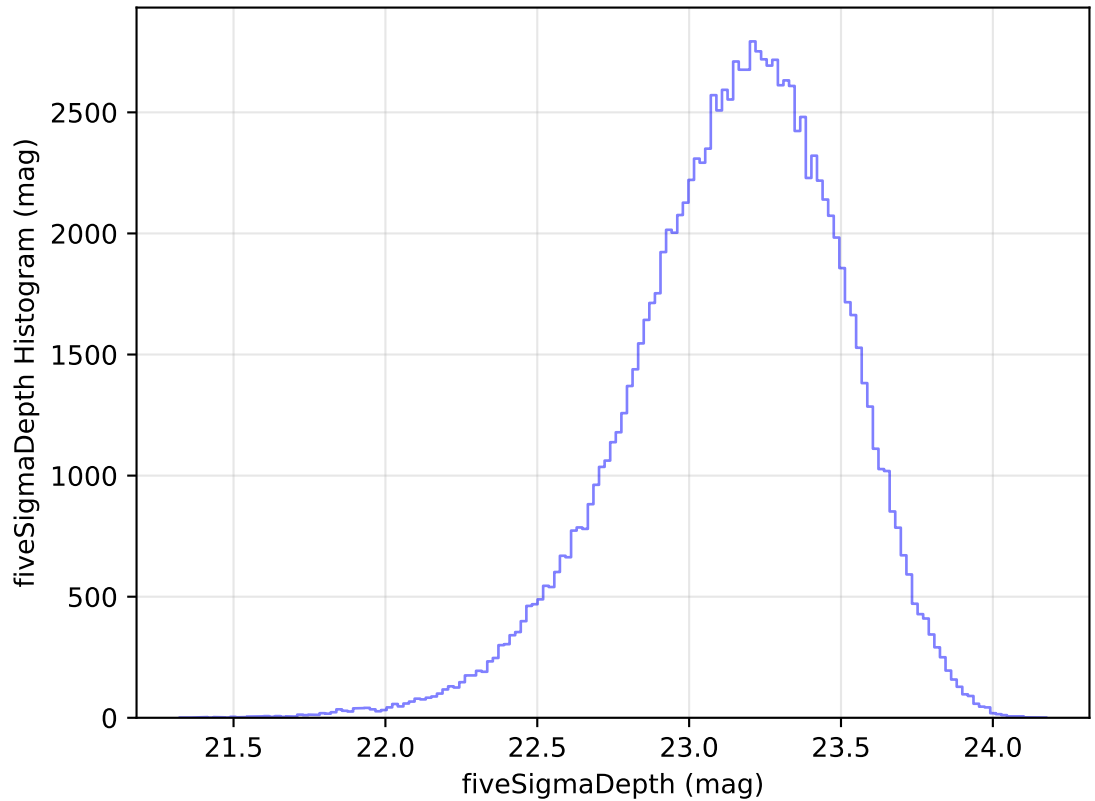
ddf_acor_sf15_lsf30_lsr10_v3.4_10yrs WFD u band: fiveSigmaDepth Histogram
