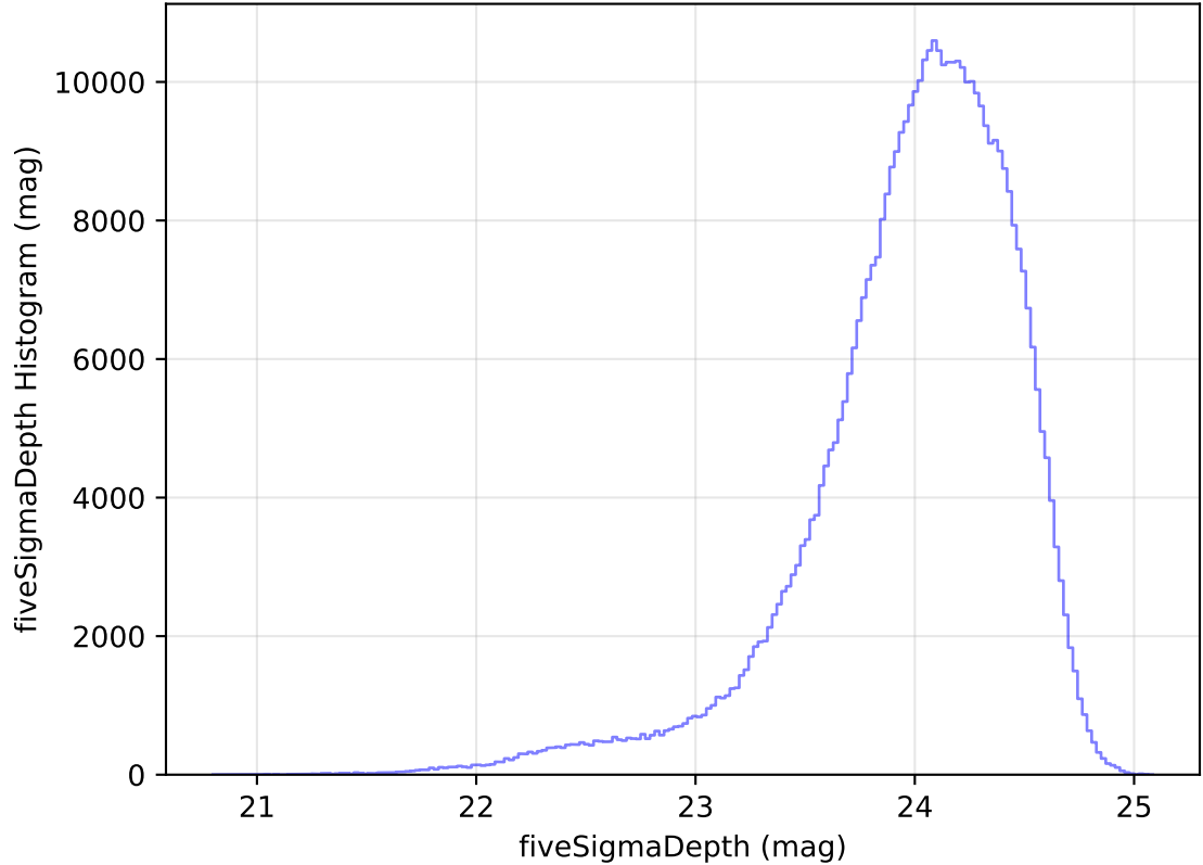
ddf_acor_sf15_lsf30_lsr10_v3.4_10yrs WFD r band: fiveSigmaDepth Histogram
