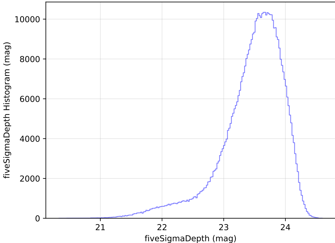
ddf_acor_sf15_lsf30_lsr10_v3.4_10yrs WFD i band: fiveSigmaDepth Histogram
