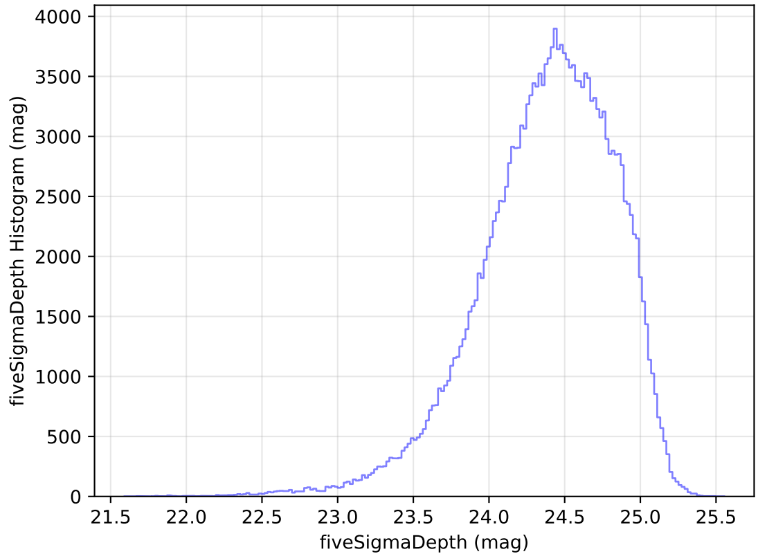
ddf_acor_sf15_lsf30_lsr10_v3.4_10yrs WFD g band: fiveSigmaDepth Histogram
