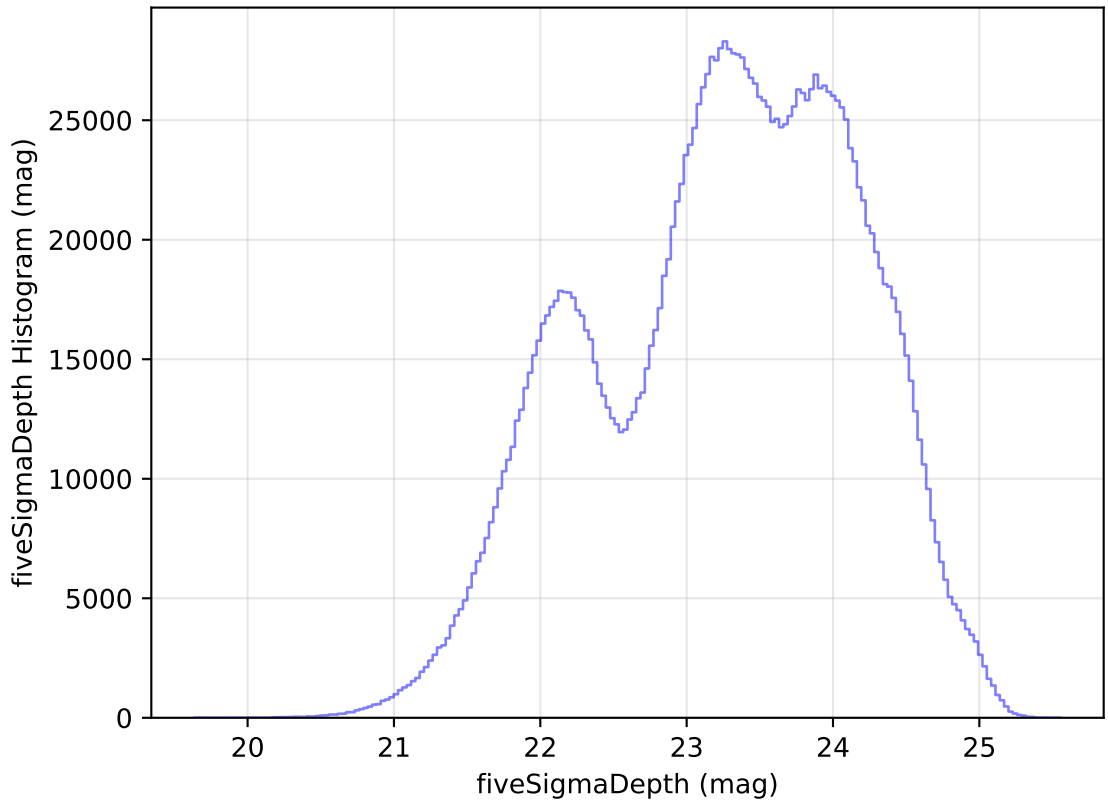
ddf_acor_sf15_lsf30_lsr10_v3.4_10yrs WFD all bands: fiveSigmaDepth Histogram
