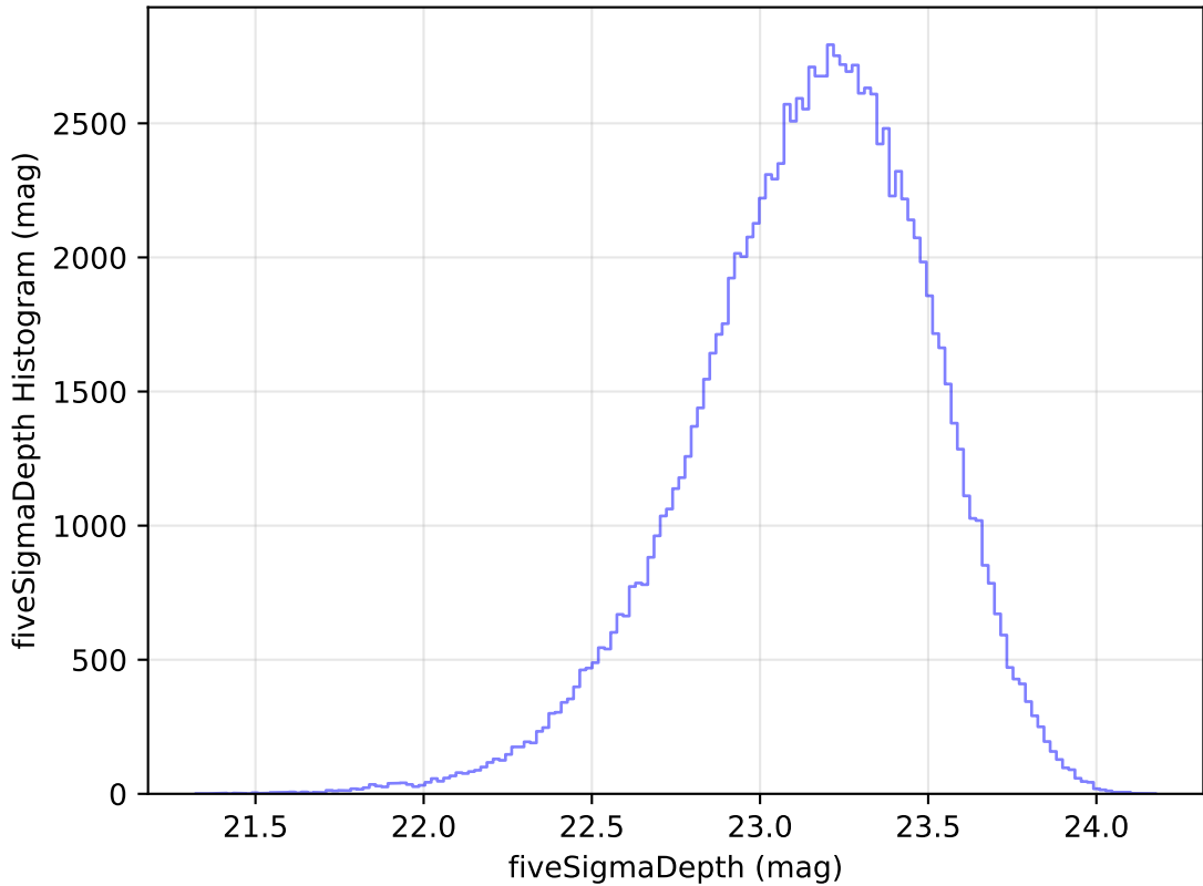
ddf_acor_sf15_lsf30_lsr10_v3.4_10yrs All sky u band: fiveSigmaDepth Histogram
