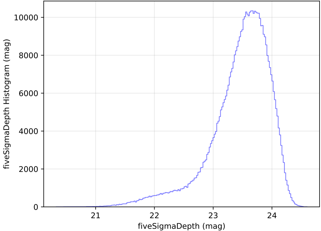
ddf_acor_sf15_lsf30_lsr10_v3.4_10yrs All sky i band: fiveSigmaDepth Histogram
