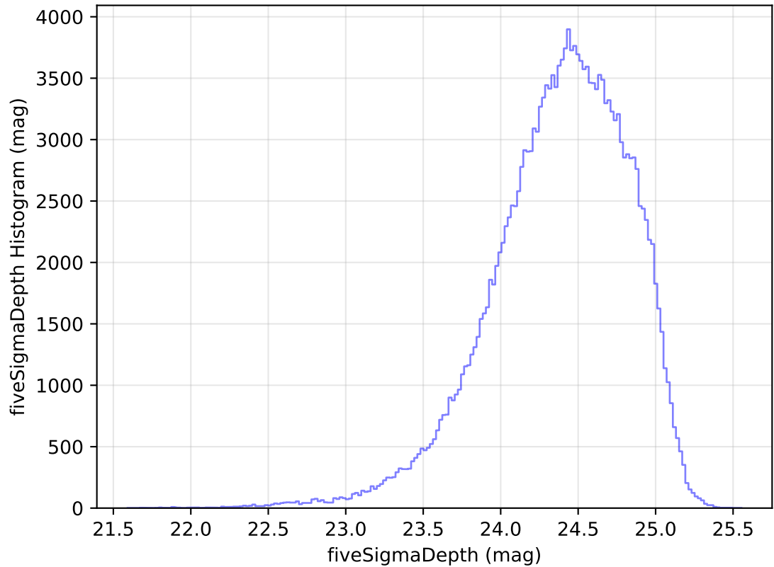
ddf_acor_sf15_lsf30_lsr10_v3.4_10yrs All sky g band: fiveSigmaDepth Histogram
