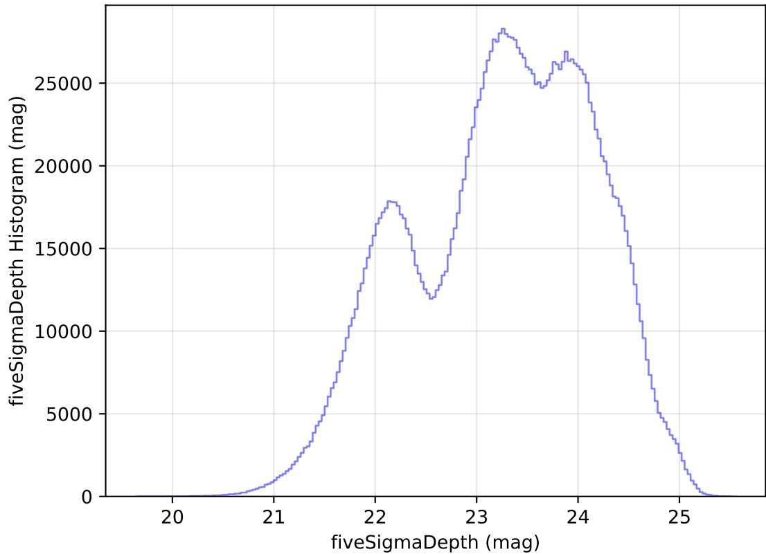
ddf_acor_sf15_lsf30_lsr10_v3.4_10yrs All sky all bands: fiveSigmaDepth Histogram
