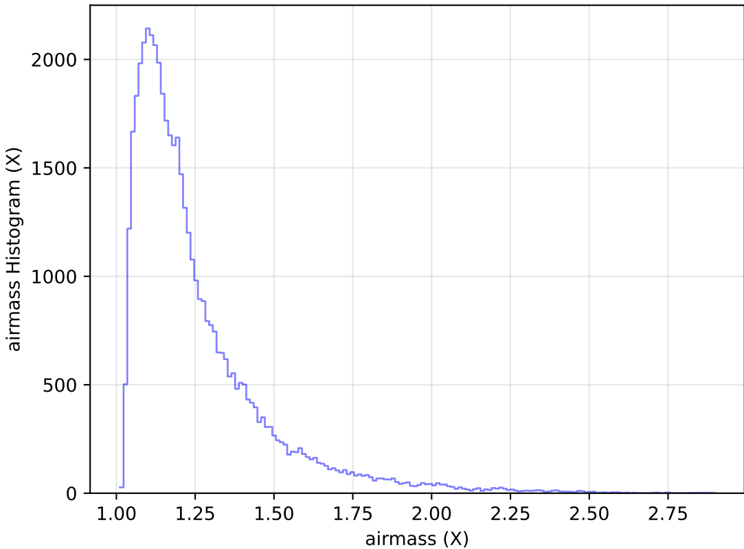
ddf_acor_sf15_lsf30_lsr10_v3.4_10yrs Yr 1 y band: airmass Histogram
