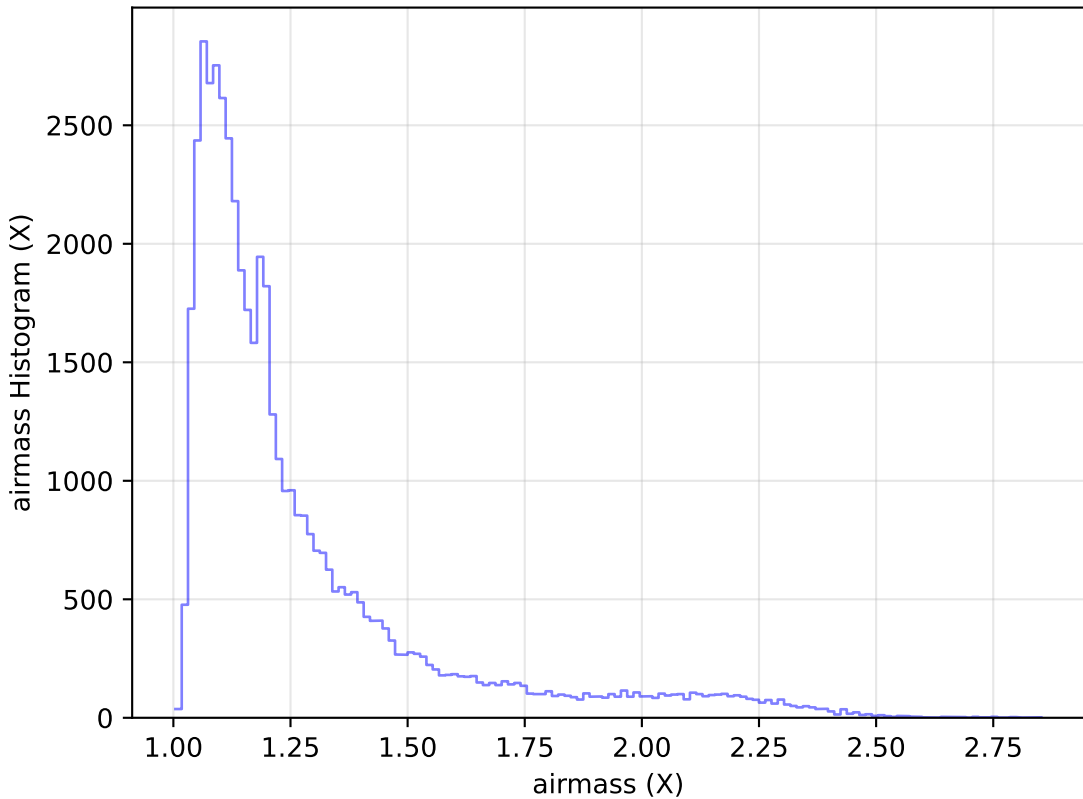
ddf_acor_sf15_lsf30_lsr10_v3.4_10yrs Yr 1 r band: airmass Histogram
